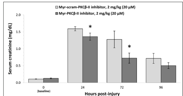
Figure 1. Serum Cr (mg/dL) in male C57BL/6J mice following bilateral renal I/R.
